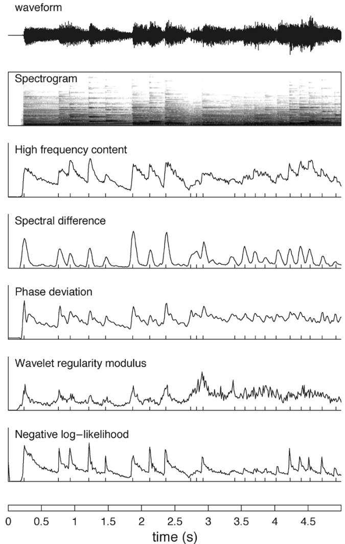
Fig. 5. Comparison of different detection functions for 5 s of a solo piano recording. From top to bottom: time-domain signal, spectrogram, high-frequency content, spectral difference, spread of the distribution of phase deviations, wavelet regularity modulus, and negative log-likelihood using an ICA model. All detection functions have been normalized to their maximum value.
