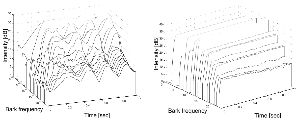
Figure 8. Sinusoid envelope representations for flute (left) and clarinet (right), playing the note C4, 261 Hz.
