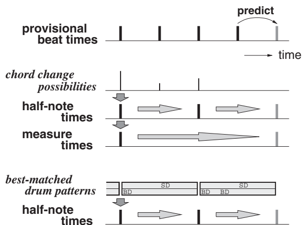
Fig. 10. Knowledge-based inferring.
