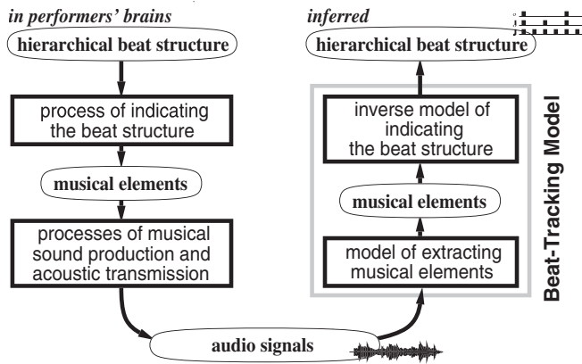
Fig. 3. Beat-tracking model.
