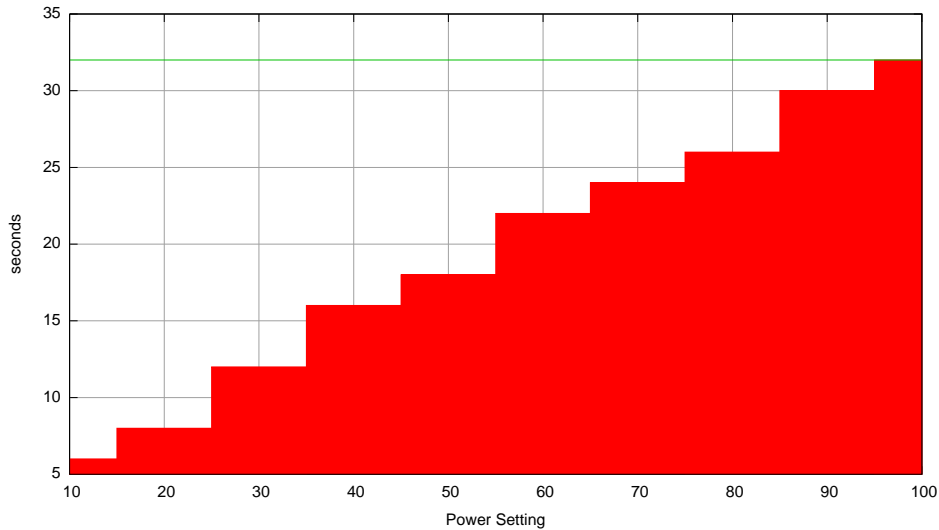
Microwave Duty Cycle
